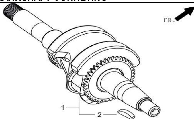
FIG.4 ROD,CRANKSHAFT CONNETING
