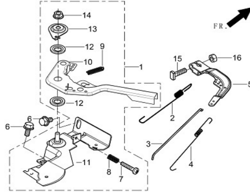
FIG.14 CONTROL ASSY, THROTTLE
