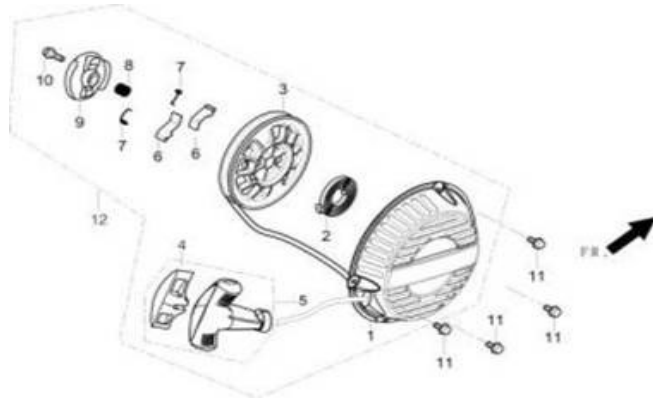
FIG.7 STARTER,RECOIL
