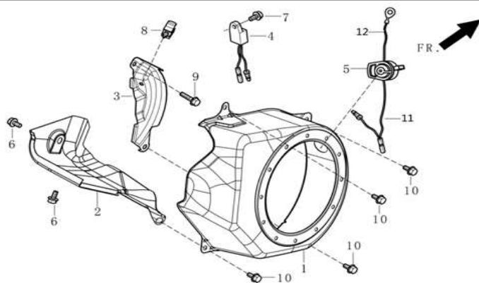
FIG.8 SHROUD / SHIELD,LOWER
