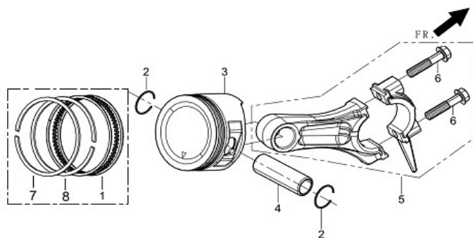
FIG.5 RING SET,OIL / ROD,CRANKSHAFT CONNECTING
