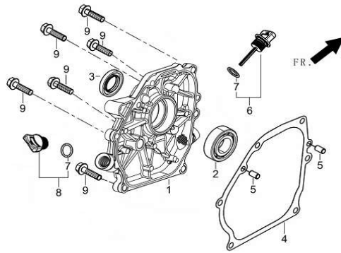
FIG.3 COVER SUB-ASSEMBLY, CRANKCASE
